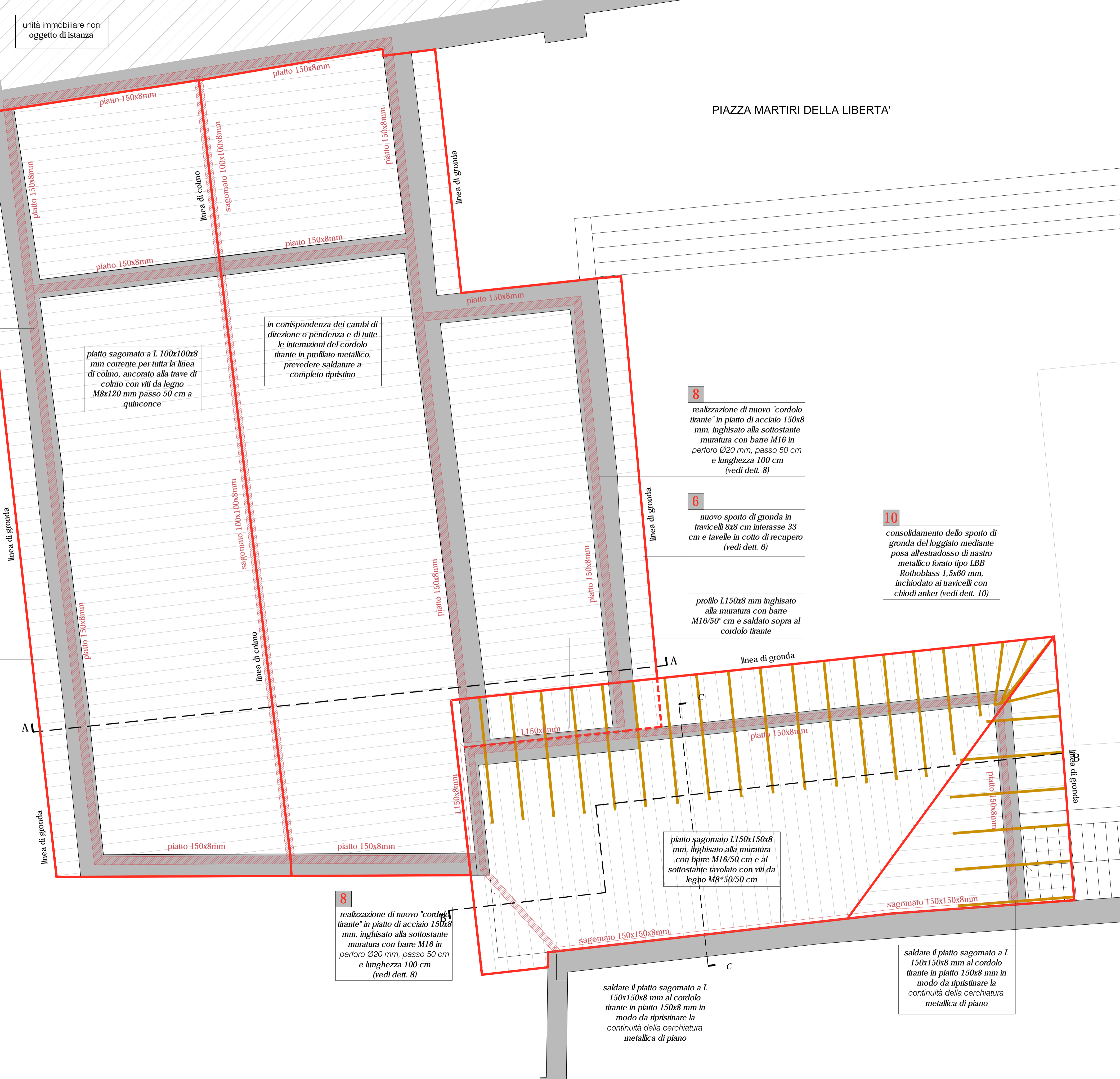
PIANTA PIANO COPERTURE
